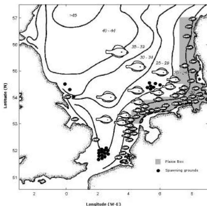
Figure 3. Location of the 'Plaice Box' and schematic representation of the distribution of plaiice in the North Sea with mean sizes (total length, in cm) given for each depth range (from Rijnsdorp, 1998, modified after Garstang 1908 and reproduced with the kind permission of the European Commission).
